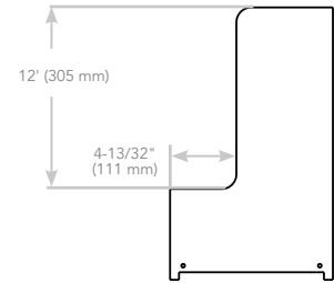
PIPE CLEARANCE DIMENSIONS (For both units)
