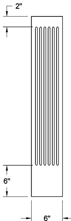
6" Fluted Filler/Base/Tall
