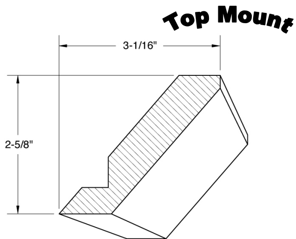
Shaker Crown 538
