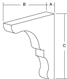
Jennings Bracket
