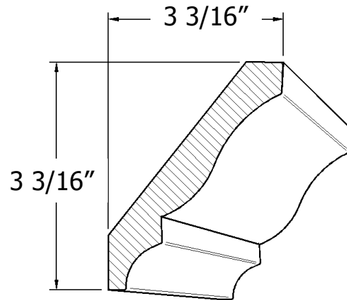
Stock Crown #19
