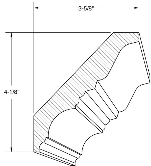
Crown 859
