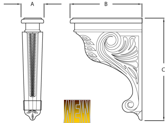
Acanthus Corbel
