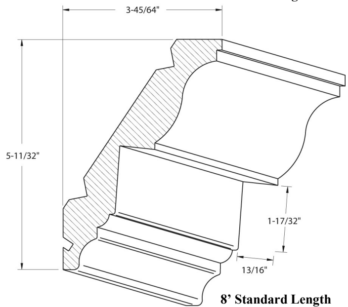
Crown 1622
