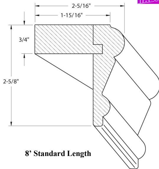
Light Rail 1619
