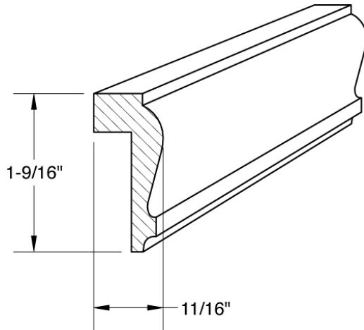
Wainscot Cap 8
