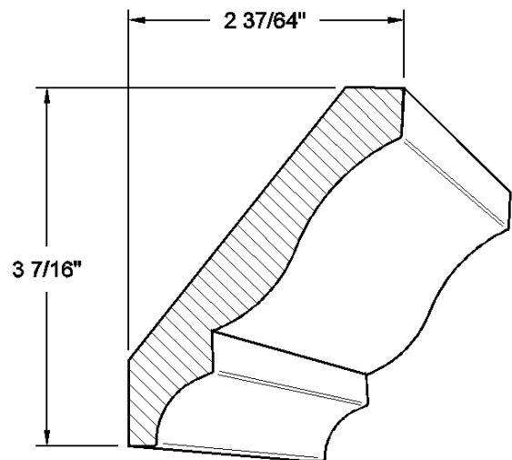
Crown #24
