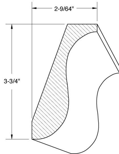
Crown 1017
