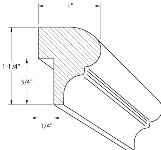
Light Rail 361
