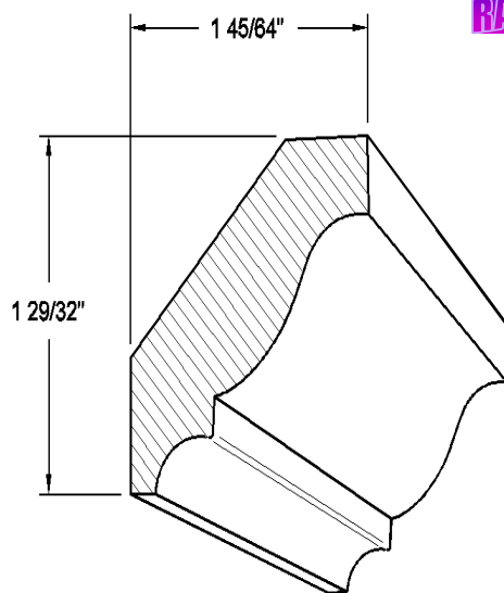
Crown #6
