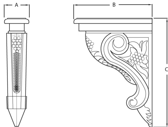
Grape Corbel
