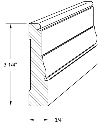
Casing 466
