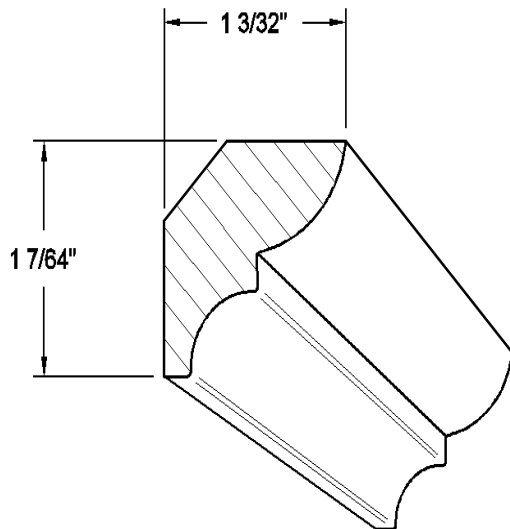
Crown # 33
