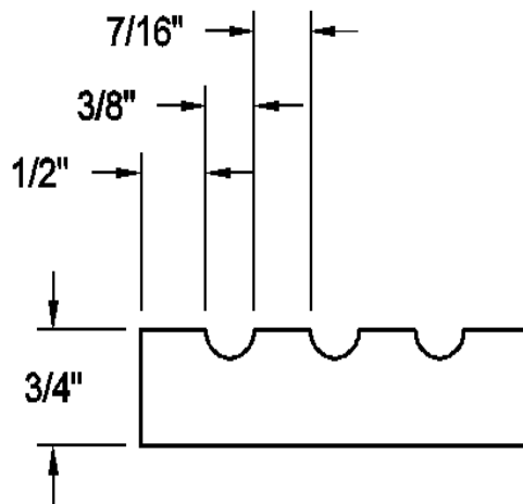
3" Fluted Filler/Wall
