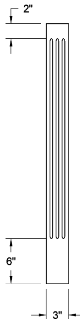
3" Fluted Filler/Base/Tall
