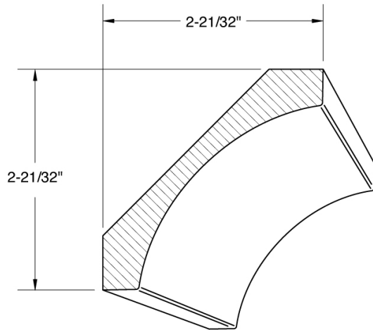
Cove Crown 2048
