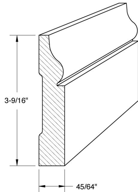
Base 2021
