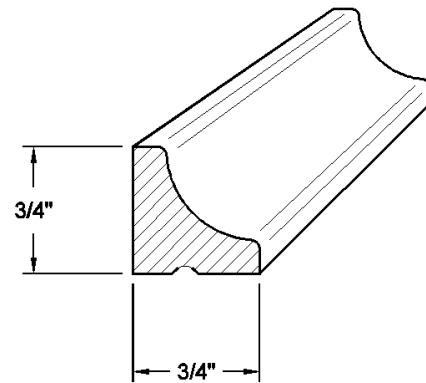
Cove 11
