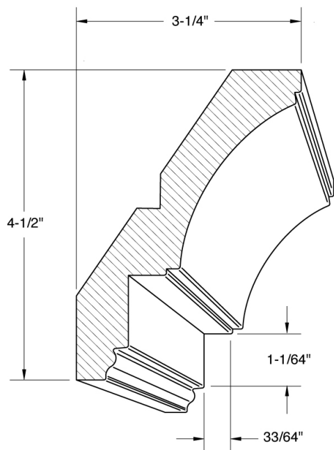
Crown 2057
