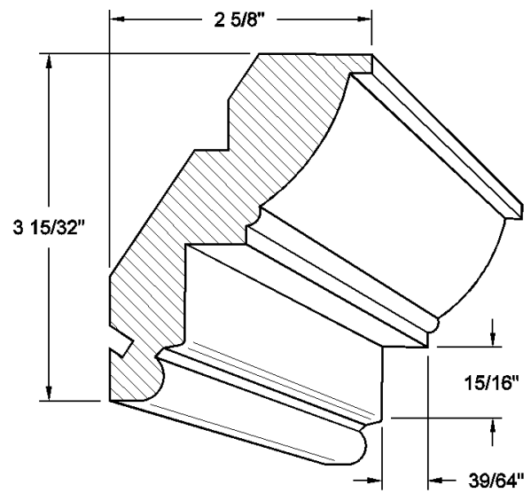
Crown #344
