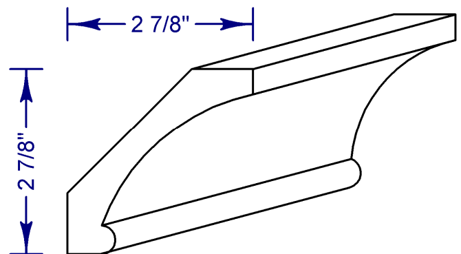
Stock Crown #48
