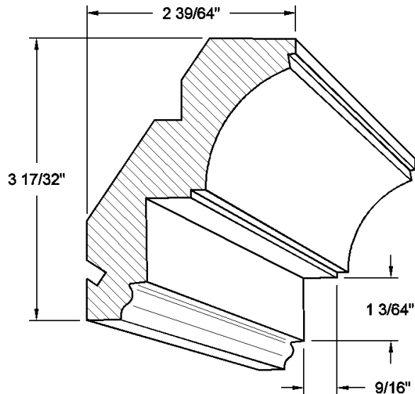
Crown #343
