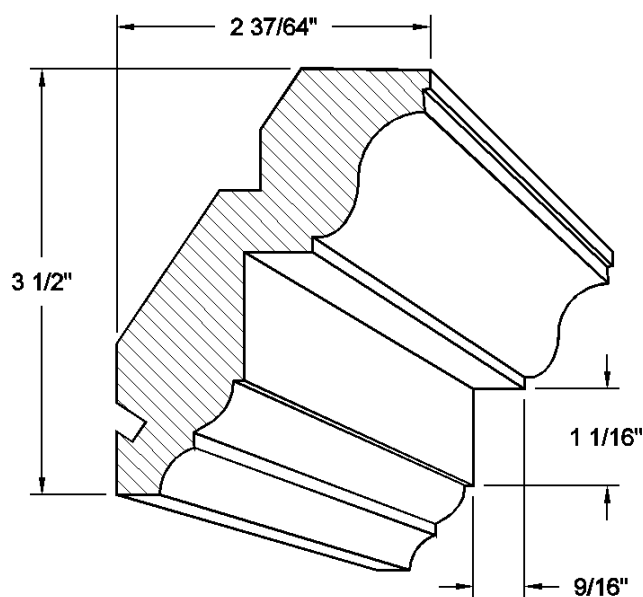
Crown # 342
