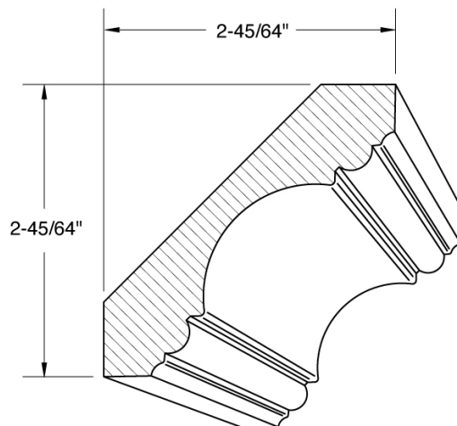
Crown 1557
