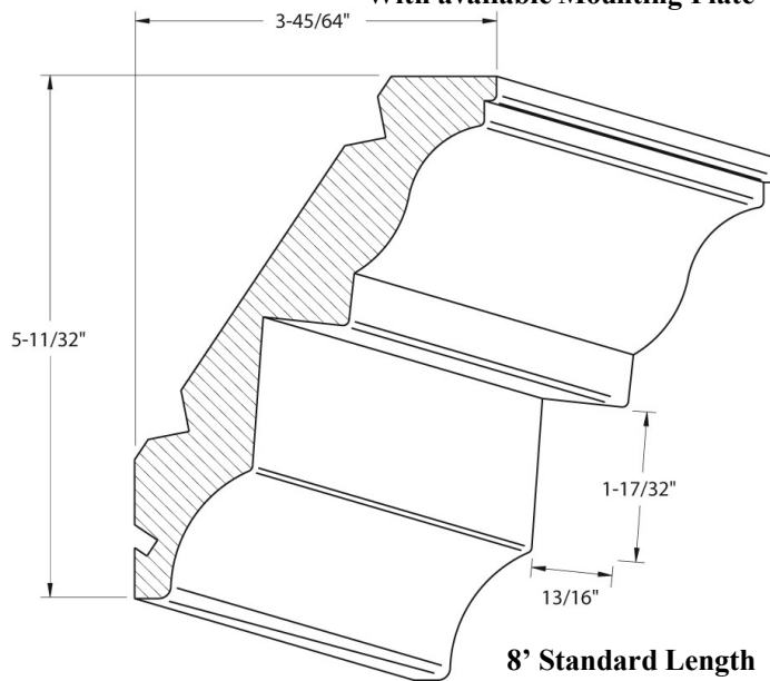
Crown 1621
