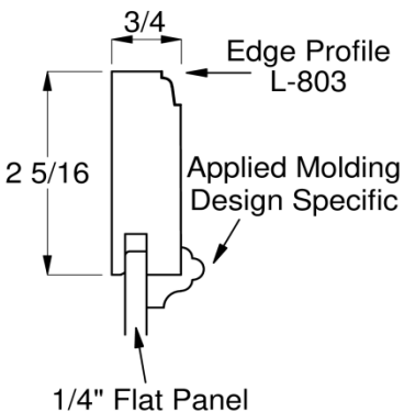
Door and Drawer Panel and Edge Profile Option
