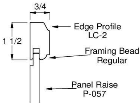
Drawer Panel Option
