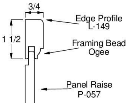
Drawer Panel Option
