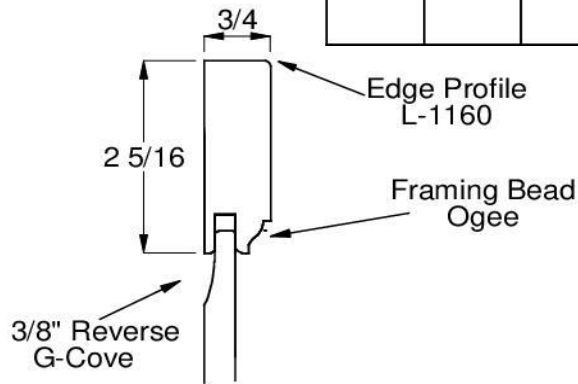
Door Panel and Edge Profile Option
