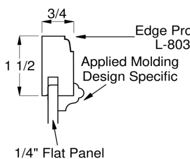
Door and Drawer Panel and Edge Profile Option
