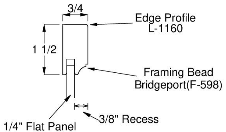
Small Drawer Front with reduced rails 'SDF'
