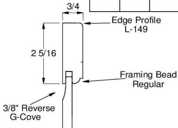
Door Panel and Edge Profile Option
