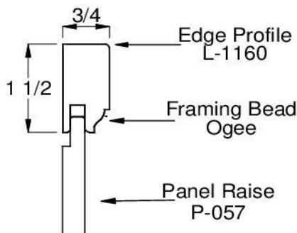
Drawer Panel and Edge Profile Options
