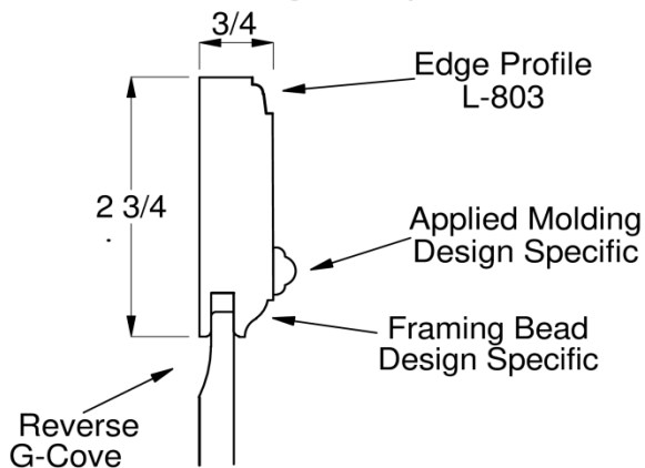
Door Edge Profile and Panel Raise Option
