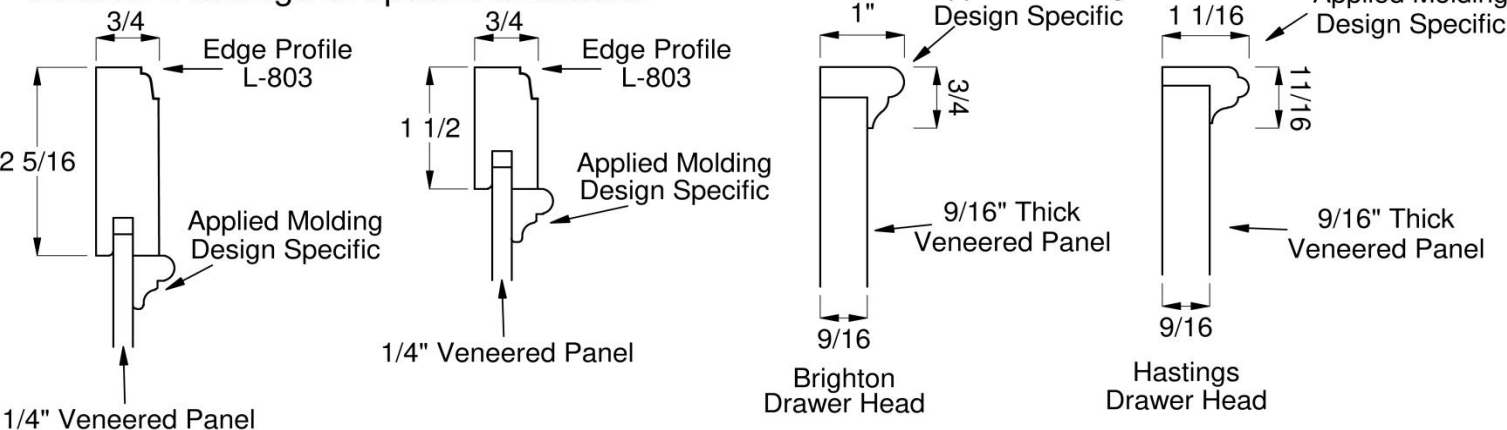
Door and Door Edge Profile Option
