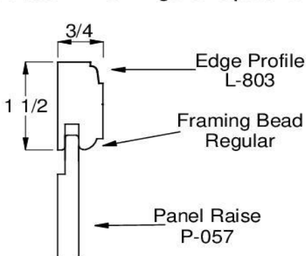
Drawer Panel Option
