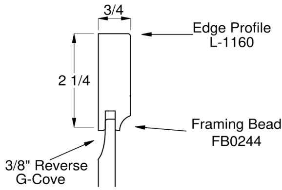
Door Panel Raise Option
