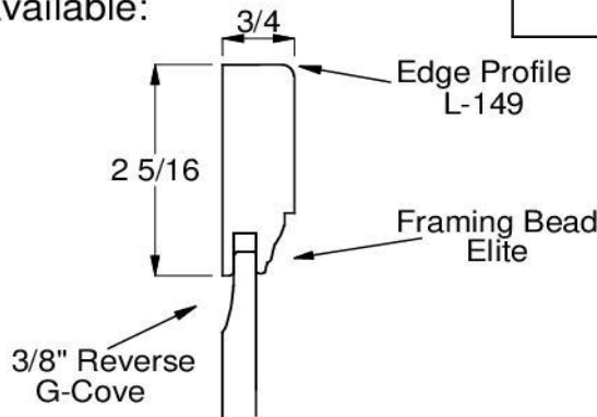
Door Panel and Edge Profile Option
