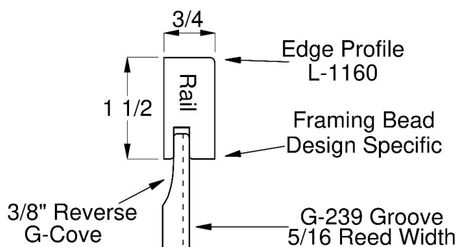
Small Drawer Front with Reduced Rails 'SDF'
