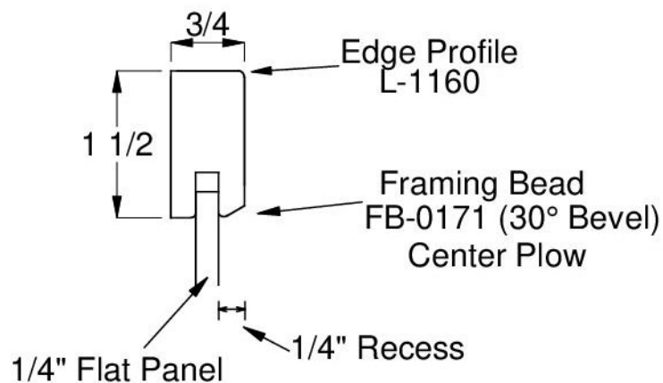
Small Drawer Front with reduced rails 'SDF'
