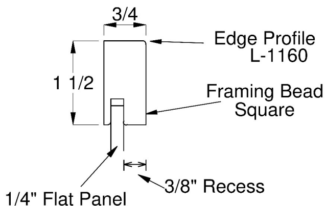
Small Drawer Front with reduced rails 'SDF'
