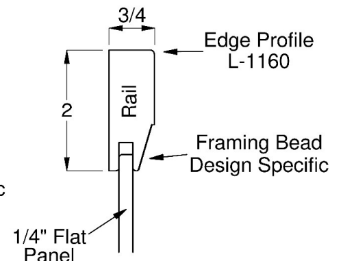
Drawer Panel Option
