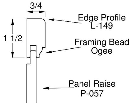
Drawer Panel Option
