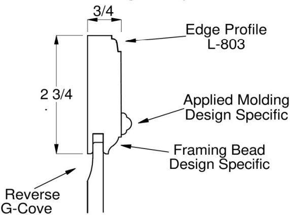
Door Edge Profile and Panel Raise Option
