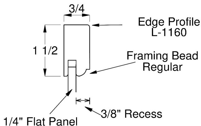
Small Drawer Front with reduced rails 'SDF'
