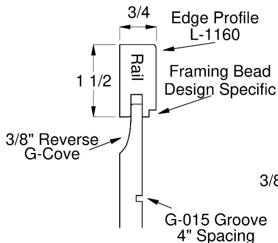
Small Drawer Front With Reduced Rails 'SDF'
