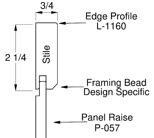
Large Drawer Front matches SDF framing and panel 'LDF'
