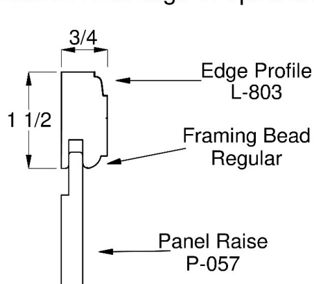
Drawer Panel Option
