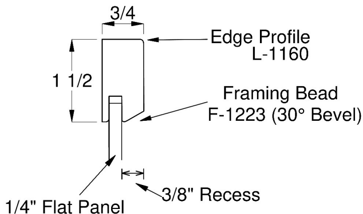
Small Drawer Front with reduced rails 'SDF'
