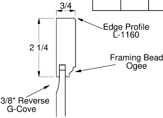
Door Panel and Edge Profile Option
